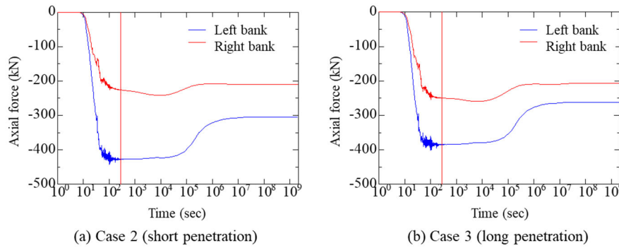
Fig. 10 Change over time in the tie rod axial force for Cases 2 and 3
