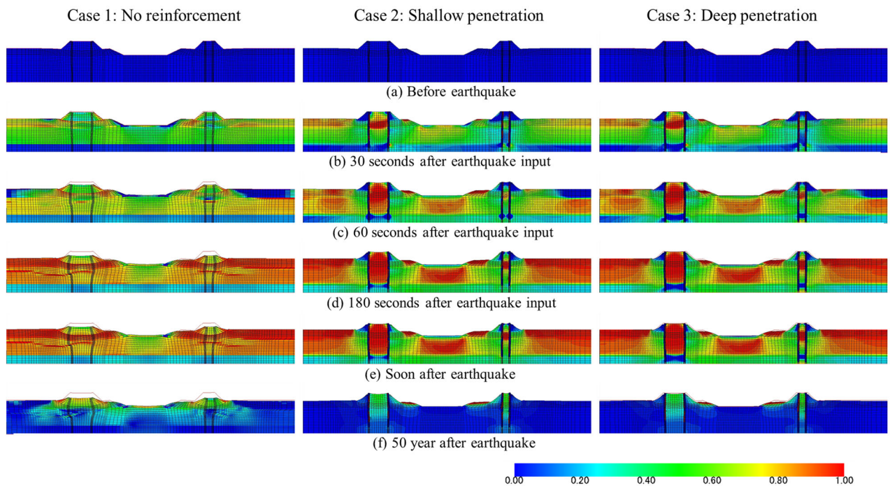
Fig. 4 Distributions of excess pore water pressure ratio
