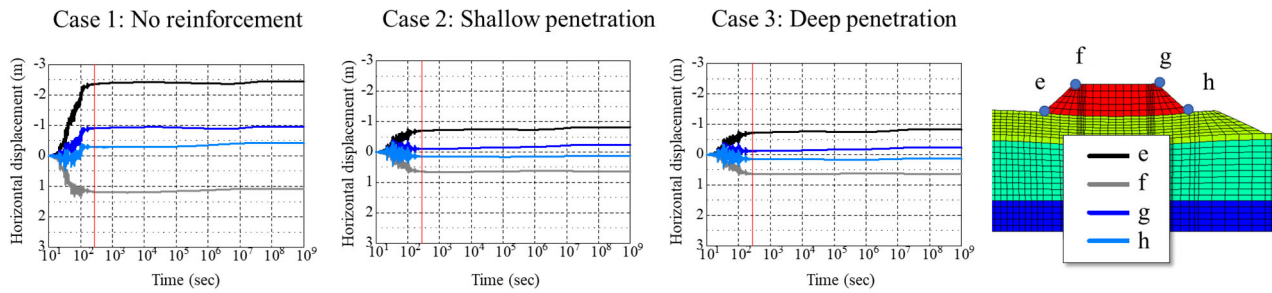
Fig. 7 Amount of horizontal displacement at the toe and shoulder of the left bank
