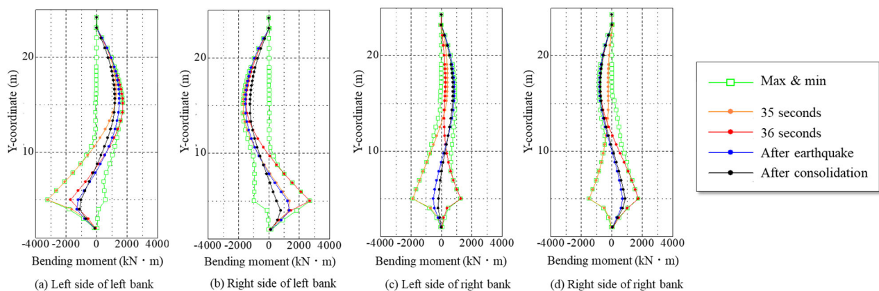
Fig. 9 Temporal changes in the bending moment in the depth direction acting on the sheet piles in Cases 3
