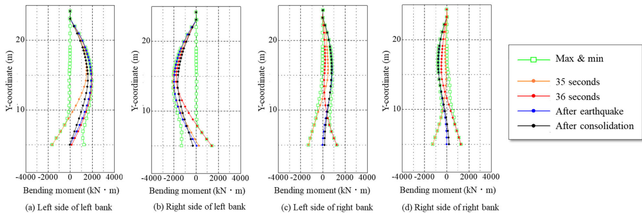
Fig. 8 Temporal changes in the bending moment in the depth direction acting on the sheet piles in Cases 2
