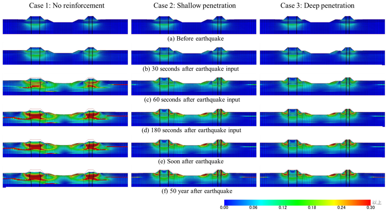
Fig.3 Distributions of shear strain
