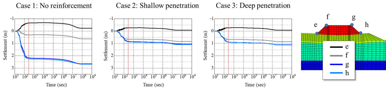
Fig.6 Amount of settlement at the toe and shoulder of the left bank
