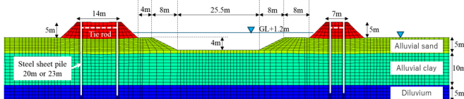
Fig. 1 Finite element mesh
